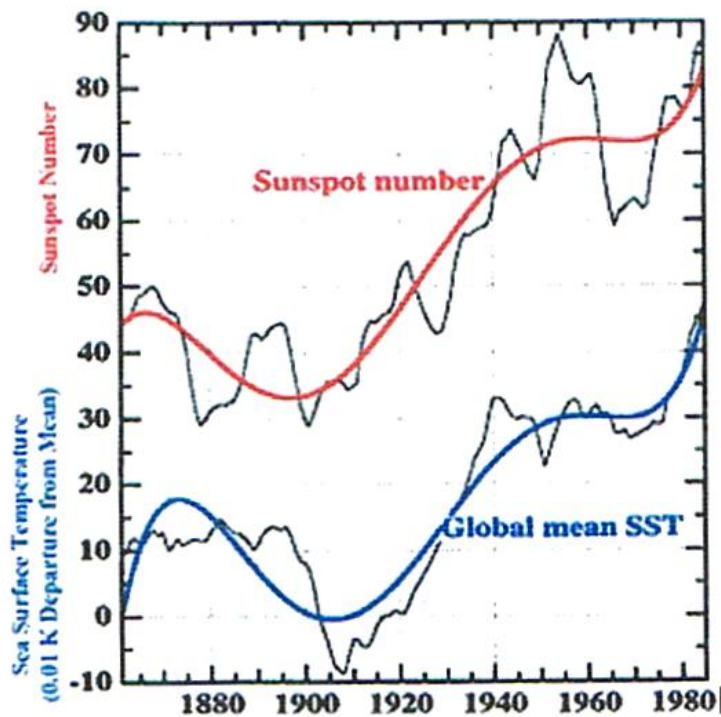
Figure 13: Global mean sea surface temperature departure from the mean versus sunspot number. Chart courtesy Peter Harris (2007)
