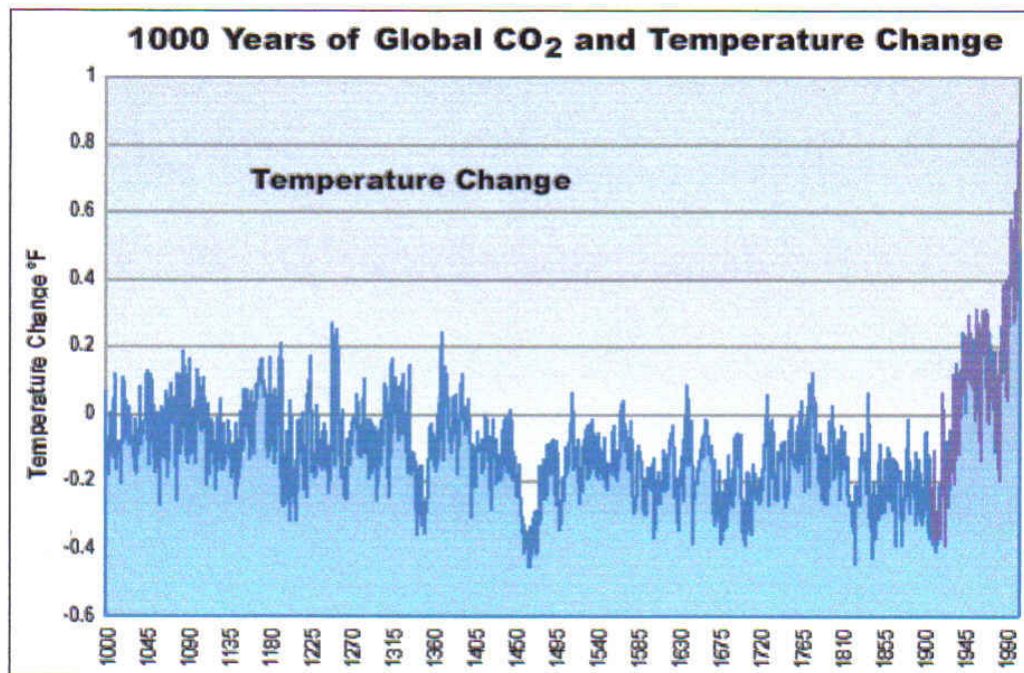
Fig.5 - The 'Hockey Stick'
