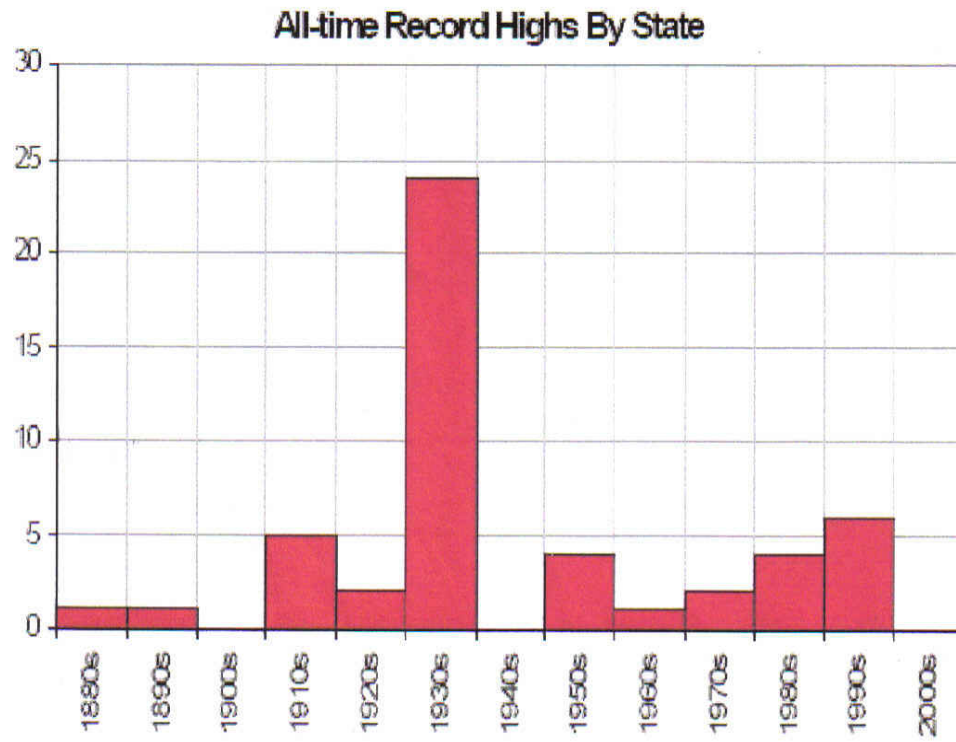
Fig. 1 State Record Temperature by Decades
