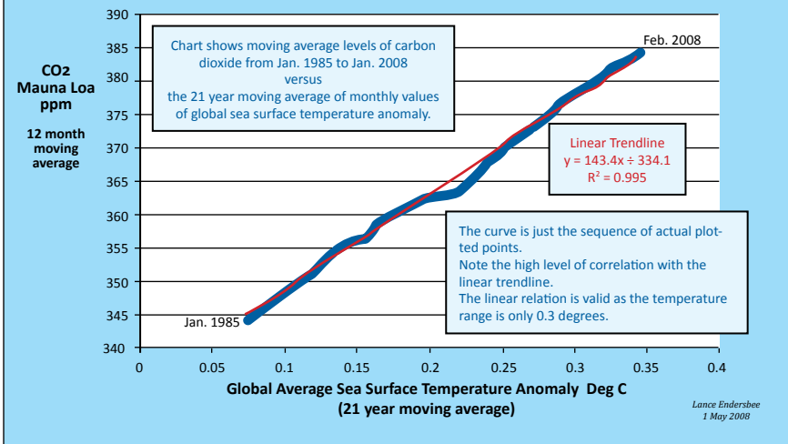
Fig. 4—Dependence of CO2 on Sea Surface Temperature
