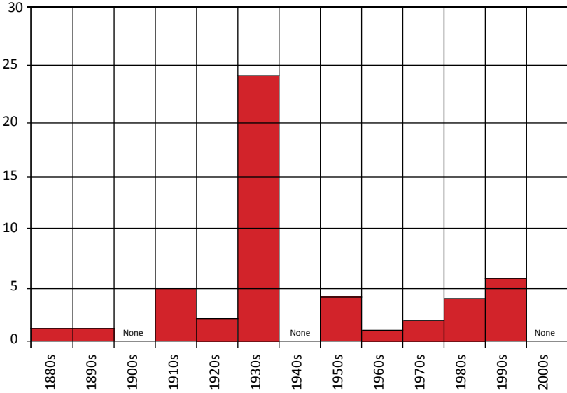
Fig. 1—State Record Temperature by Decades
