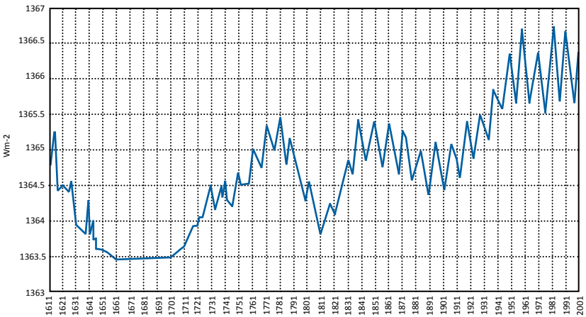
Fig. 2—Total Solar Irradiance 1611 to 2001
