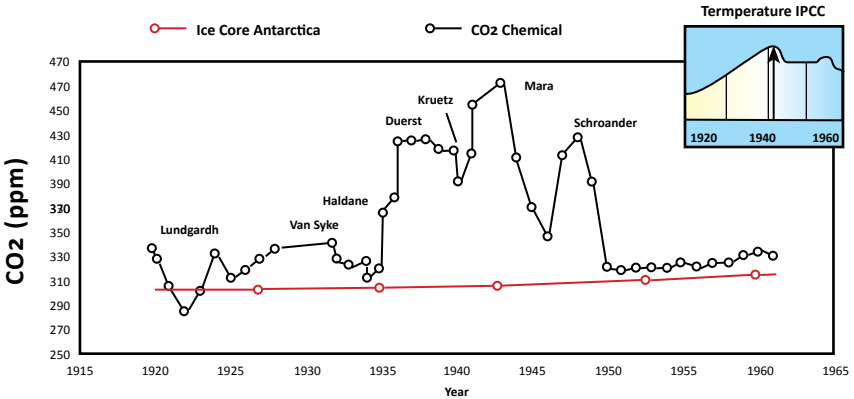
Fig. 11—Beck's CO2 Data vs. Ice Core Data
