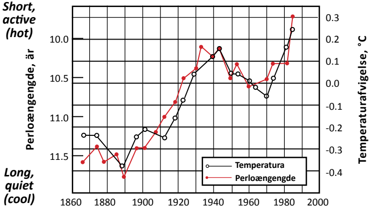
Fig. 8—Sunspot Cycle Length vs. Temperature
