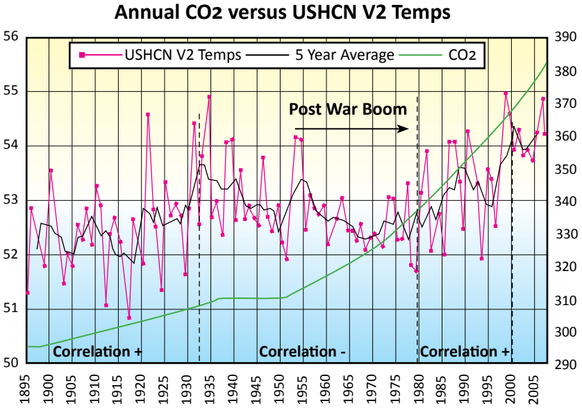
Fig. 7—Does CO2 Correlate with Air Temperature?
