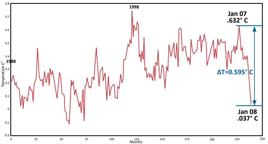
Fig. 3—Biggest Temperature Drop in One Year?
