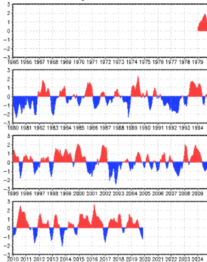
Standardized 3-Month Running Mean AAO Index Through November 2019
