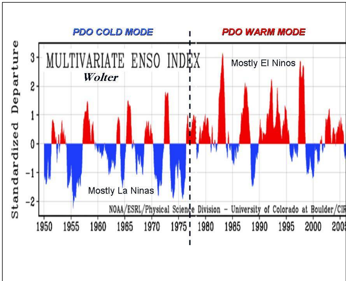
Figure 3: Wolter's Multivariate ENSO Index (MEI) since 1950. The plot starts in the early stages of a cold mode (1947 to 1977) and ends in the latter declining phases of the warm phase (1978-?). Note the increased frequency of La Nina in the cold mode of the PDO and El Nino in the warm mode.
