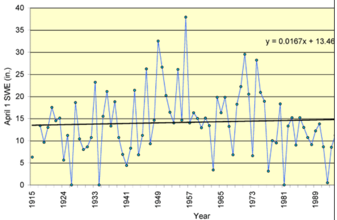
Bumping Lake WA April 1 SWE 1915-2003
