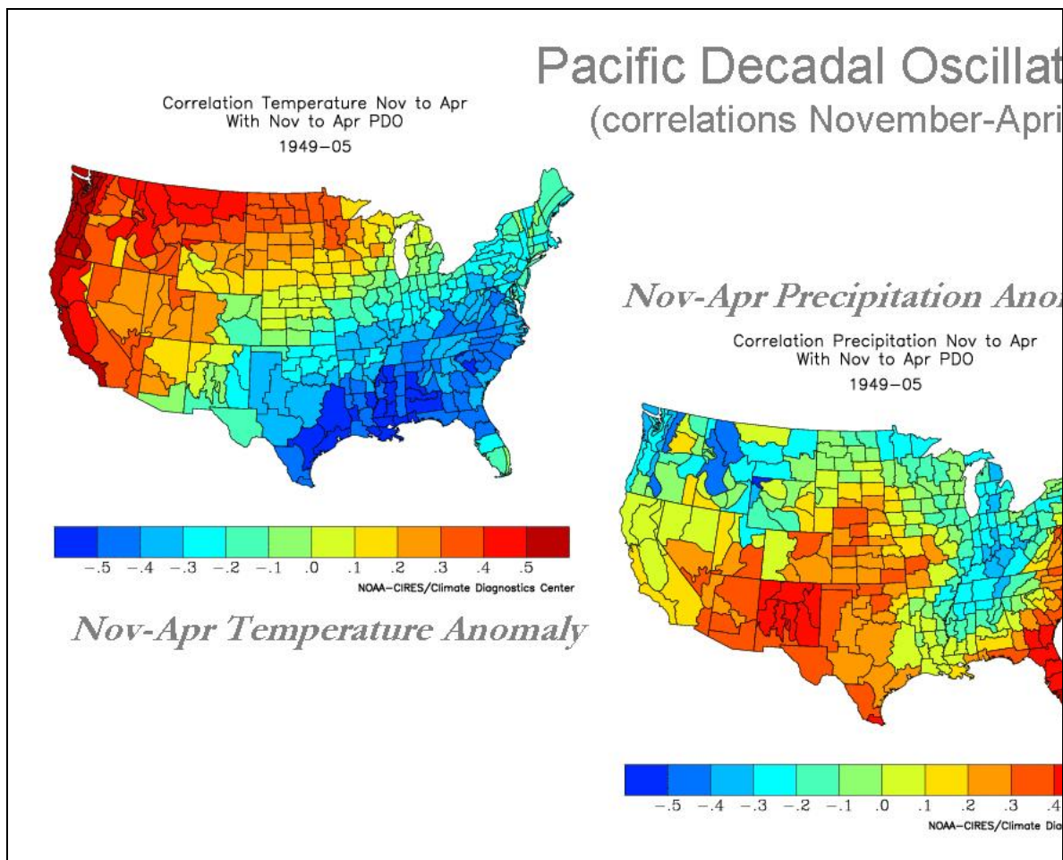
Figure 2: Correlations of Temperatures and Precipitation November to April with the PDO. In the wet season (the heart of the snow season) for the west (November to April), correlations with the positive PDO suggest warm and dry conditions in the northwest and wet conditions to the south.
