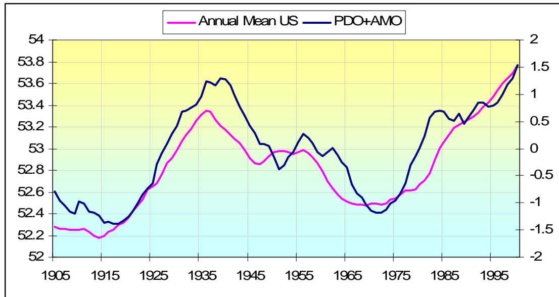
Figure 9: AMO+PDO (standardized and then added) and the US annual mean temperatures (11 year running mean). The two agree with an r -squared of 0.86
