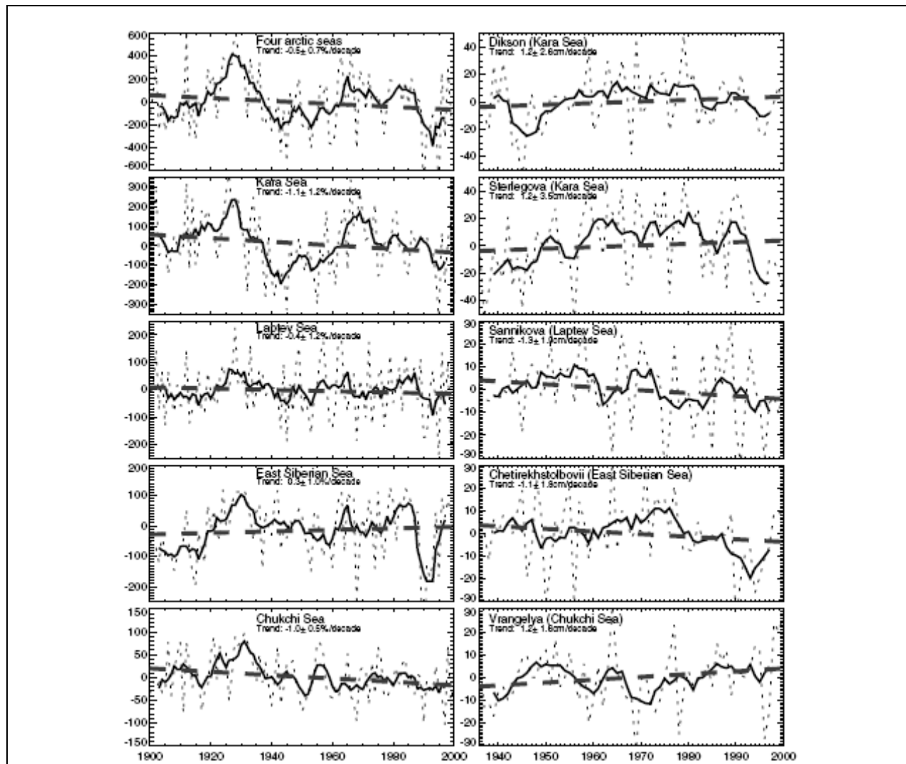
Figure 13: (Left) Time series of August ice-extent anomalies (1000 km²) in four arctic seas. (Right) Time series of annual maximum fast-ice thickness anomalies (cm) at five locations. The plot shows annual means (dotted), six-year running means (solid), and linear trends at the quoted 95% level (dashed).
