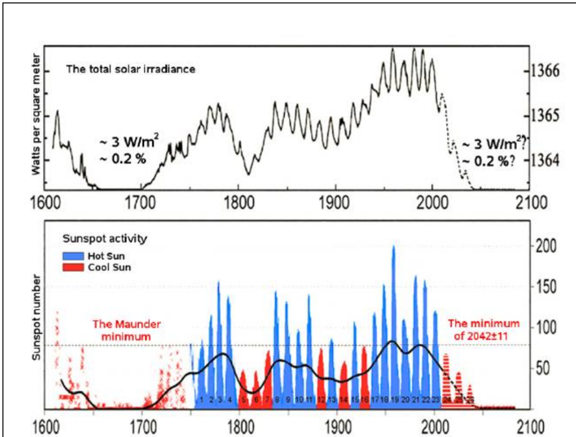
Figure 22. Habibullo Abdussamatov, Dr. Sc. Head of the Pulkovo Observatory has projected a decline in upcoming cycles to maunder minima levels.
