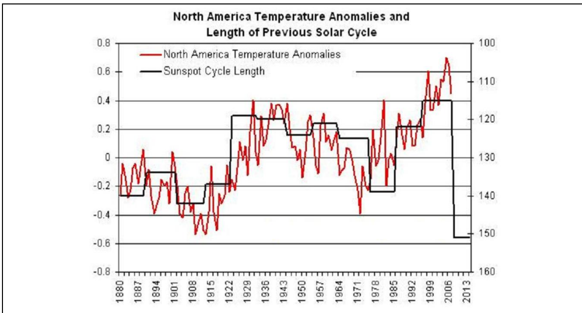
Figure 19. Historically, the North American temperatures have correlated well with solar cycle length. Note the rapid increase in length for the cycle 23, implying an upcoming cooling.
