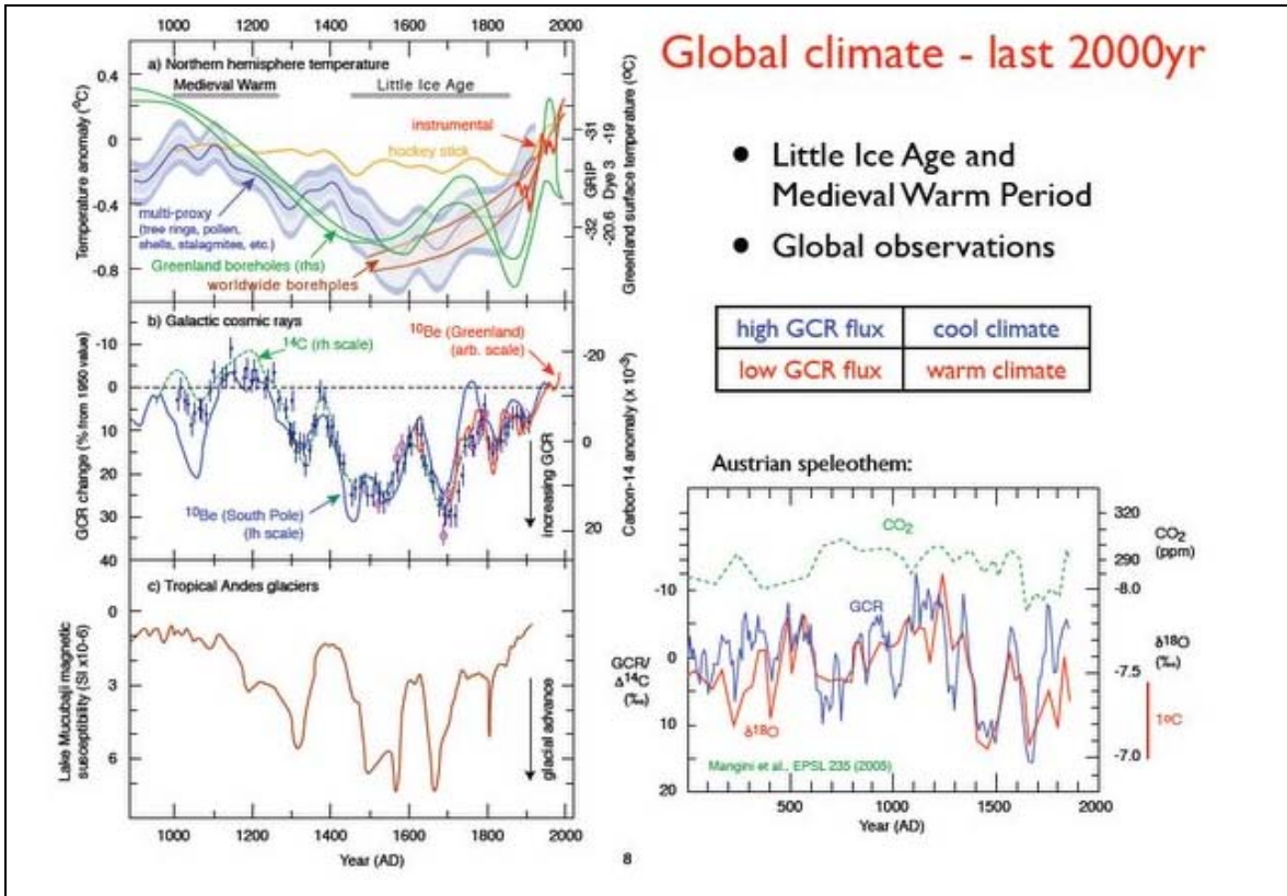
Figure 15: Jasper Kirkby of CERN show excellent correlations of galactic cosmic rays and temperatures for the Northern Hemisphere, Greenland, Tropical Andes and Austria.
