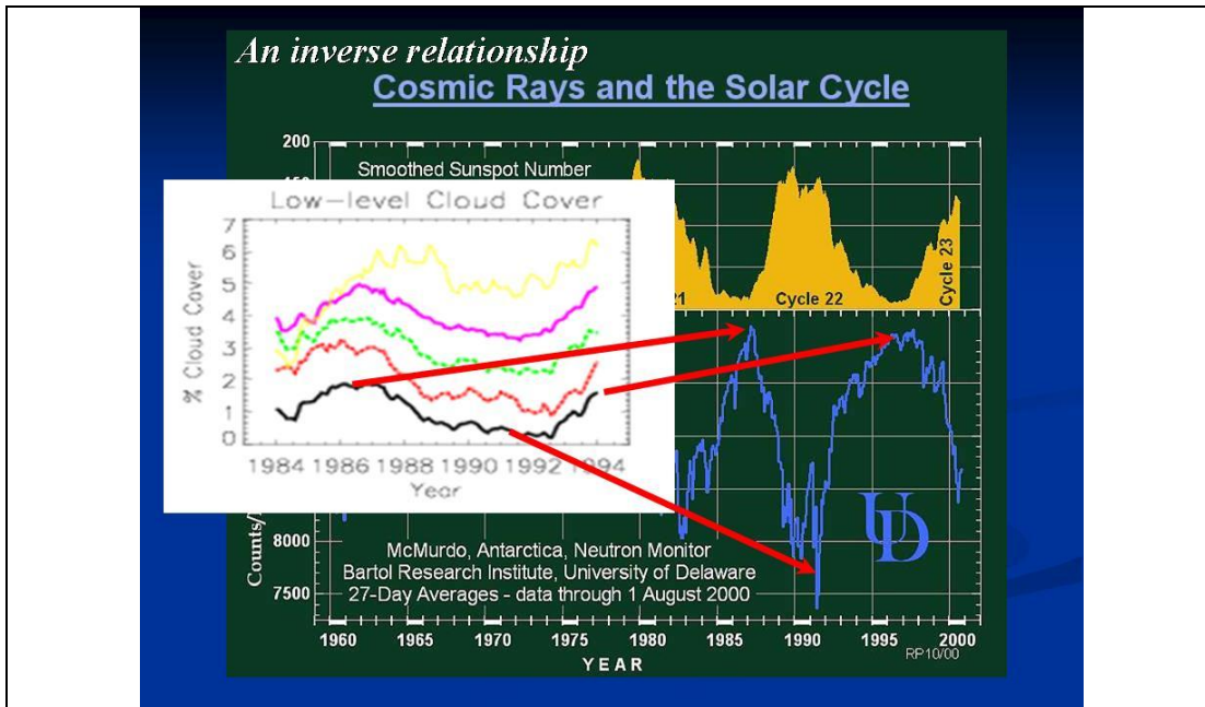
Figure 12: Cosmic ray neutrons are inversely proportional to solar activity and directly proportional to low cloudiness (from Palle-Bago and Butler 2002 )
