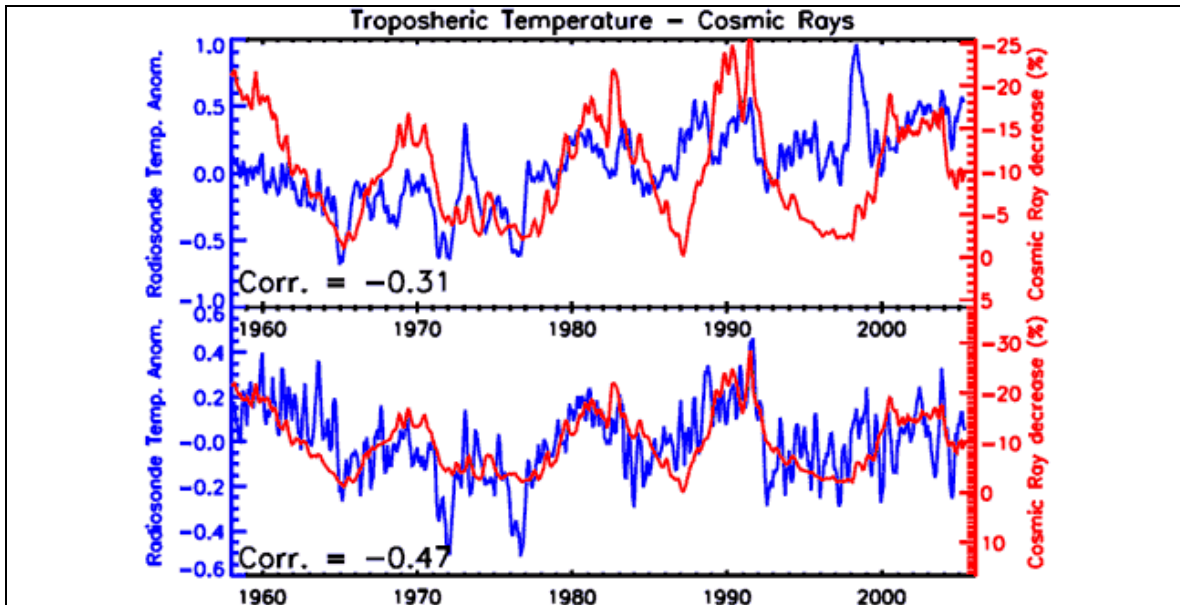
Figure 13: Tropospheric cosmic rays versus radiosonde temperature anomalies raw and bottom filtered and detrended (Henrik Svensmark and Eigil Friis-Christensen)
