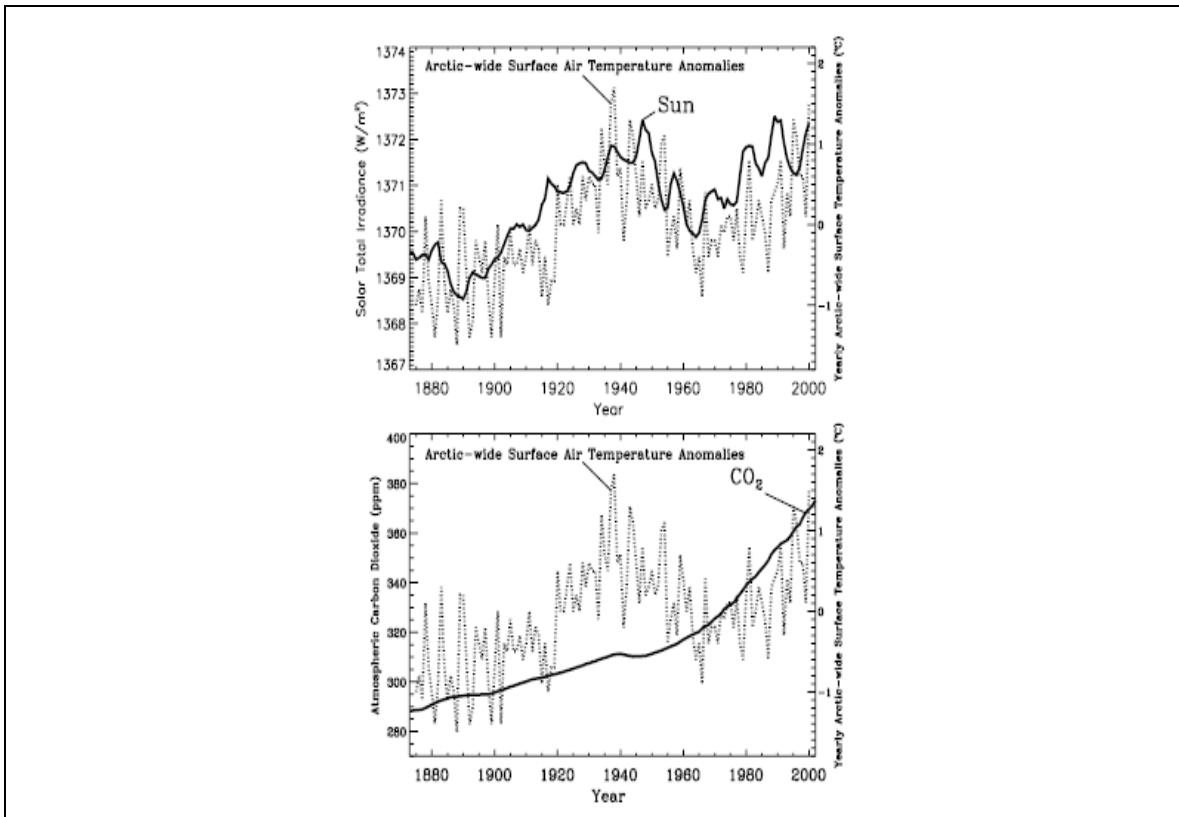
Figure 3. Arctic Basin wide air temperatures (Polyokov) correlated with Hoyt Schatten Total Solar Irradiance (TSI) and with annual average CO 2 (Soon 2005)
