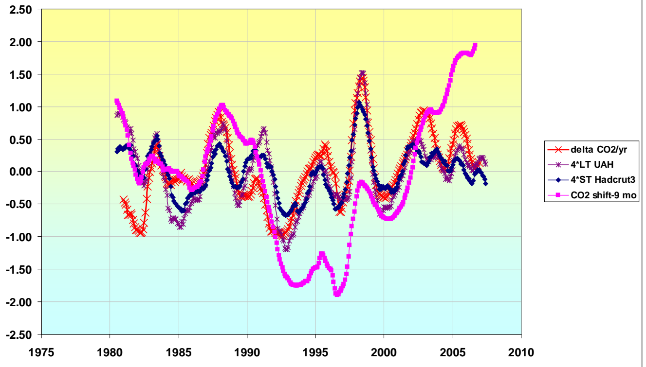
Fig. 4 - ST & LT temp, delta CO2/year & CO2 vs. time, all Running Means, all deTrend
