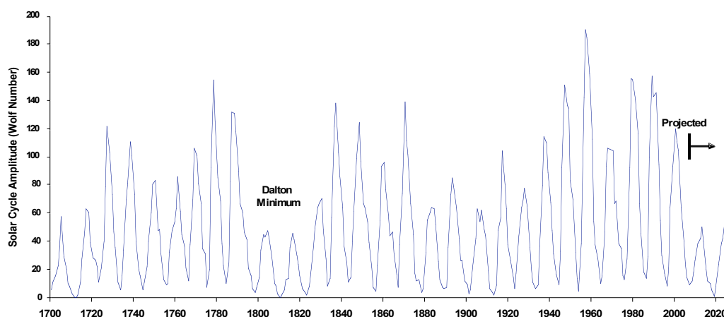
Figure 10: Sunspot Cycles 1700 - 2030
