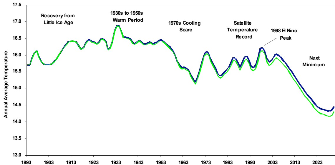
Figure 26: Calculated Anthropogenic Contribution to Atmospheric Temperature 1893 - 2030
