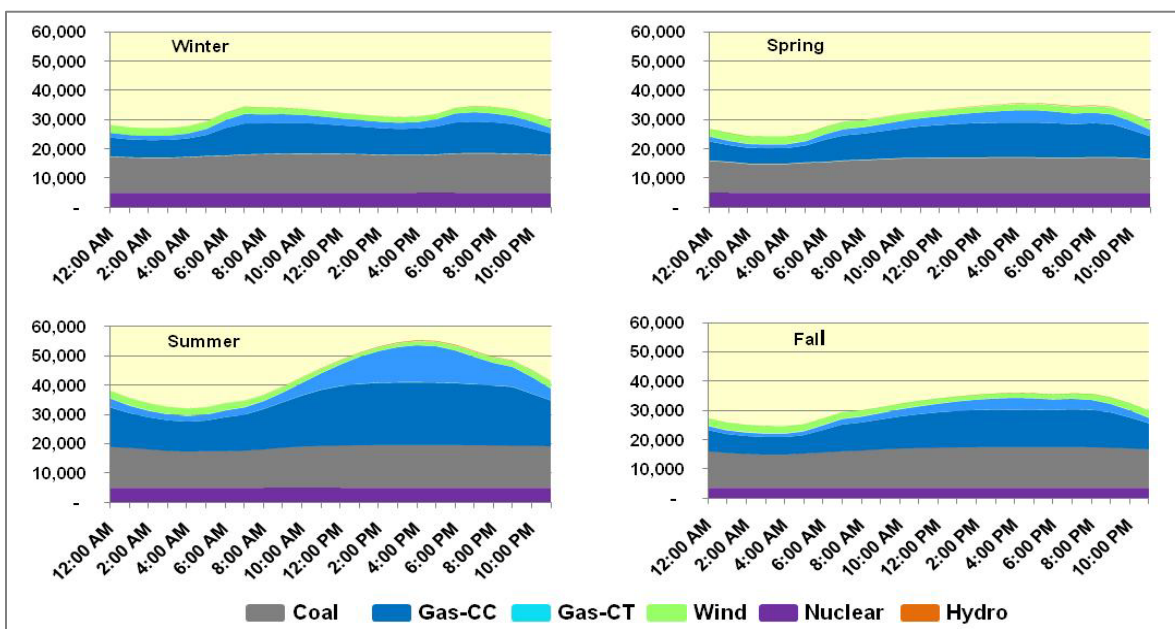
Figure VI-5 ERCOT 2009 Average Hourly Generation by Fuel Type & Season (MW)
