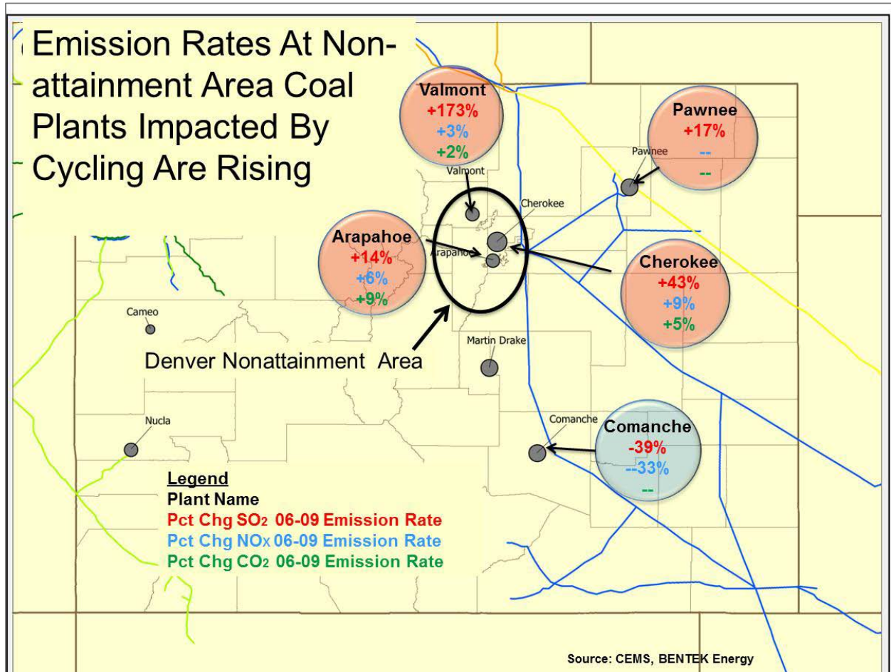
Figure I-1 Denver Non-attainment Area Plants Have Experienced Higher Emission Rates Since 2006
